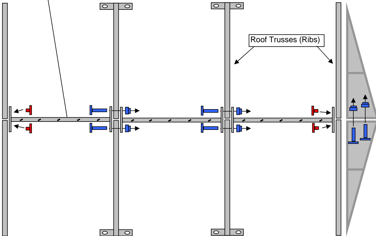
Top view of roof truss assembly
