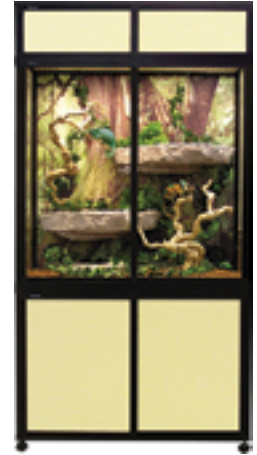
HR14 REPTILE CAGE – 36”H x 36”L x 24”D H2 HR15 REPTILE CAGE – 30”H x 30”L x 18”D H2 Similar Enclosure Pictured, Exact Not Shown
