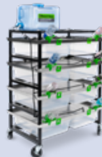
2 Section (4 level) Double Wide RODENT VERSA-RACK (QTY 8 - V-35 TUBS) Rack Height (Incl. Casters): 44.679" Rack Footprint: 33.912" X 20.884" Tub Size: 5.375" X 20" X 15"
